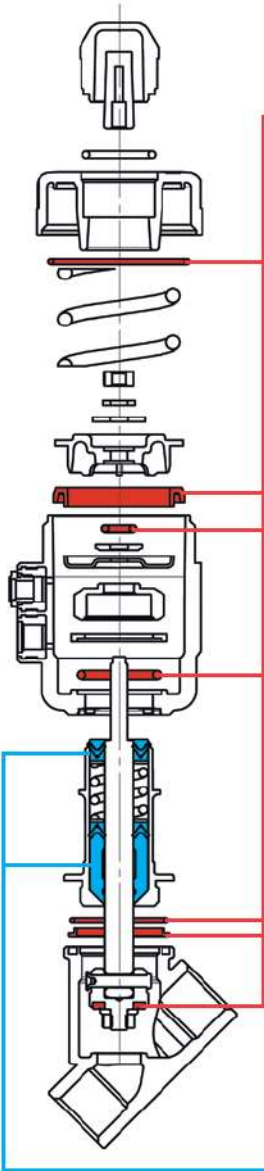
Normally Closed
