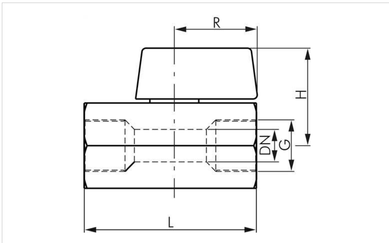
Drawing: Female thread
