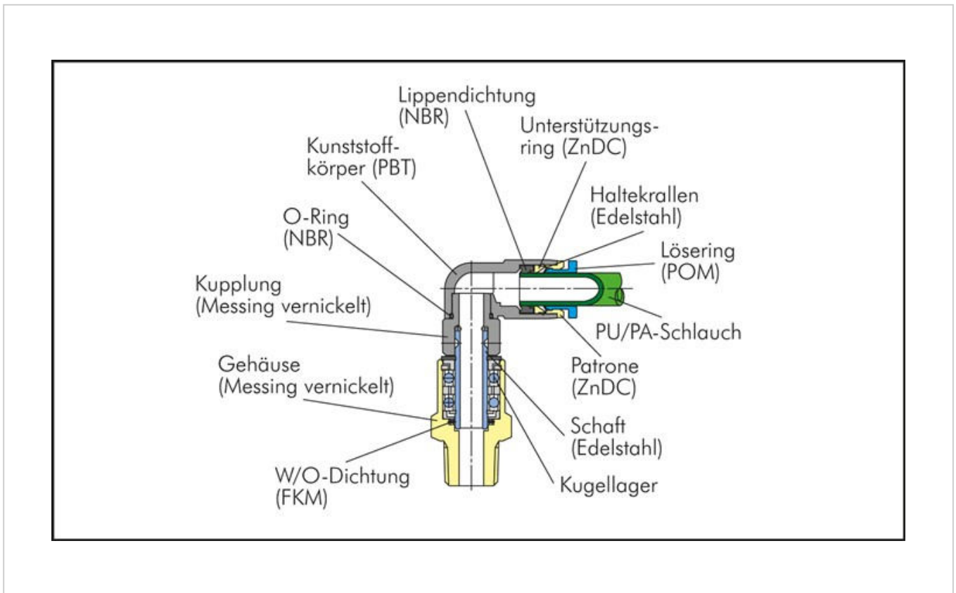
Drawing: Structure of quick swivel joint
